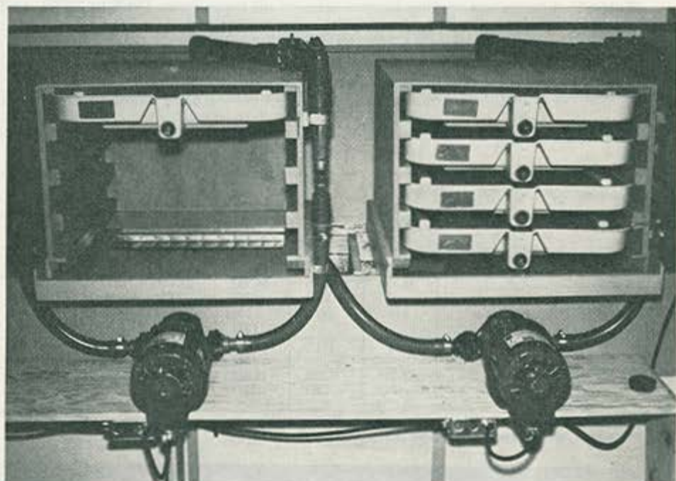
Experimental apparatus for evaluation of controlled water reuse in trays containing trout eggs. Pumps in foreground circulate water over the trays, each of which may contain up to 20,000 trout eggs for hatching.
